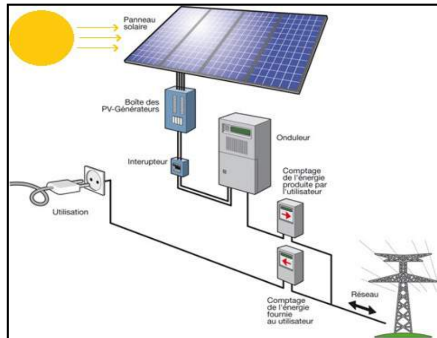
Figure 11 : Operating diagram of a solar PV plant
